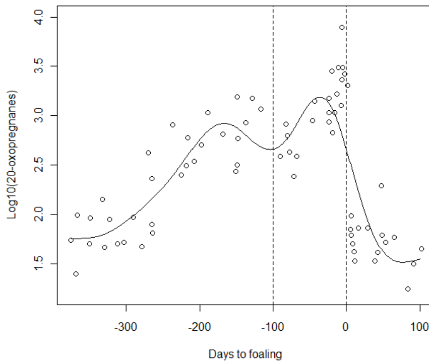
Figure 1: Log transformed concentrations of faecal 20-oxopregnanes (ng/g DW) in plains zebra mares before and after foaling.
