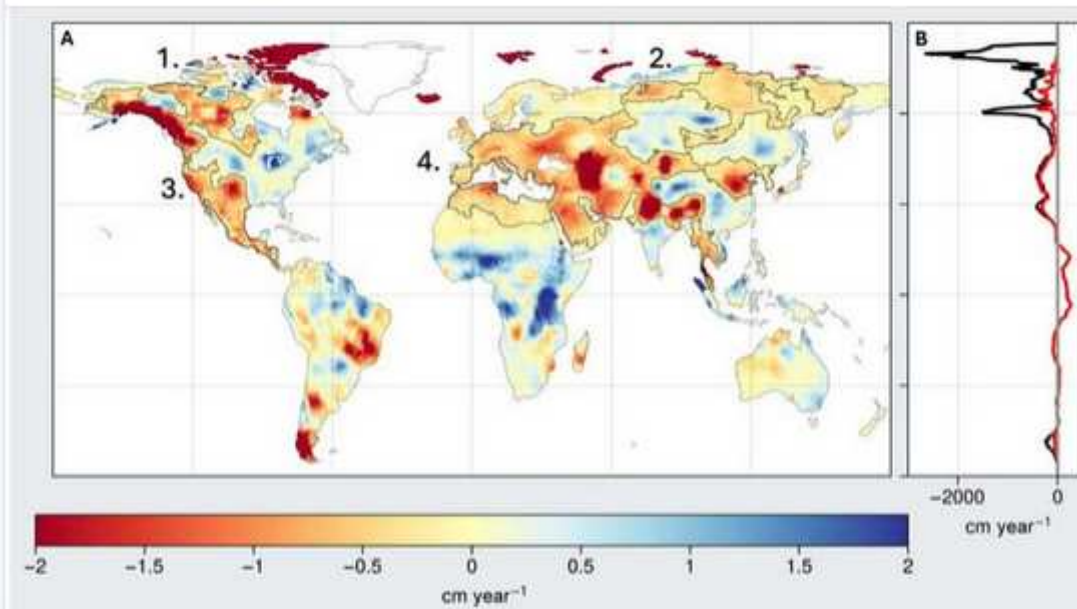
Fig. 1. Global map of long-term TWS trends from GRACE/FO.
