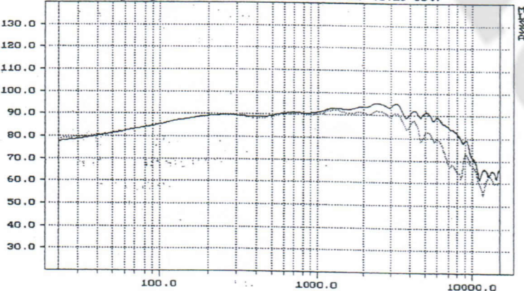
Sensitivity Mag - dB SPL/watt (8.0-ohm load) (0.18 oct)
