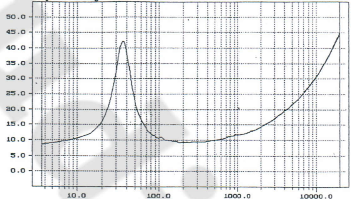
Impedance Magnitude - ohms
