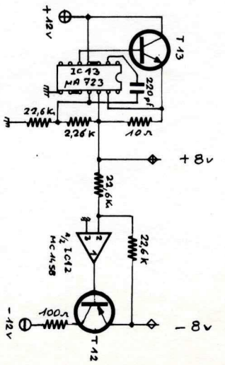
REFERENCES ±8V VCO
