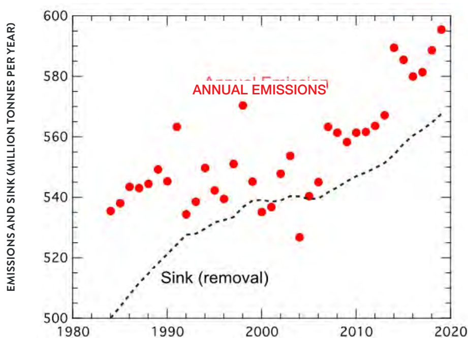
Figure 1.2 Estimated global methane emissions and sinks (removals), 1984–2019, million tonnes per year
