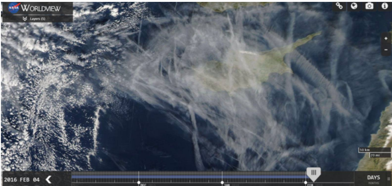
Figure 1 NASA satellite image over Cyprus, 4 Feb. 2016
