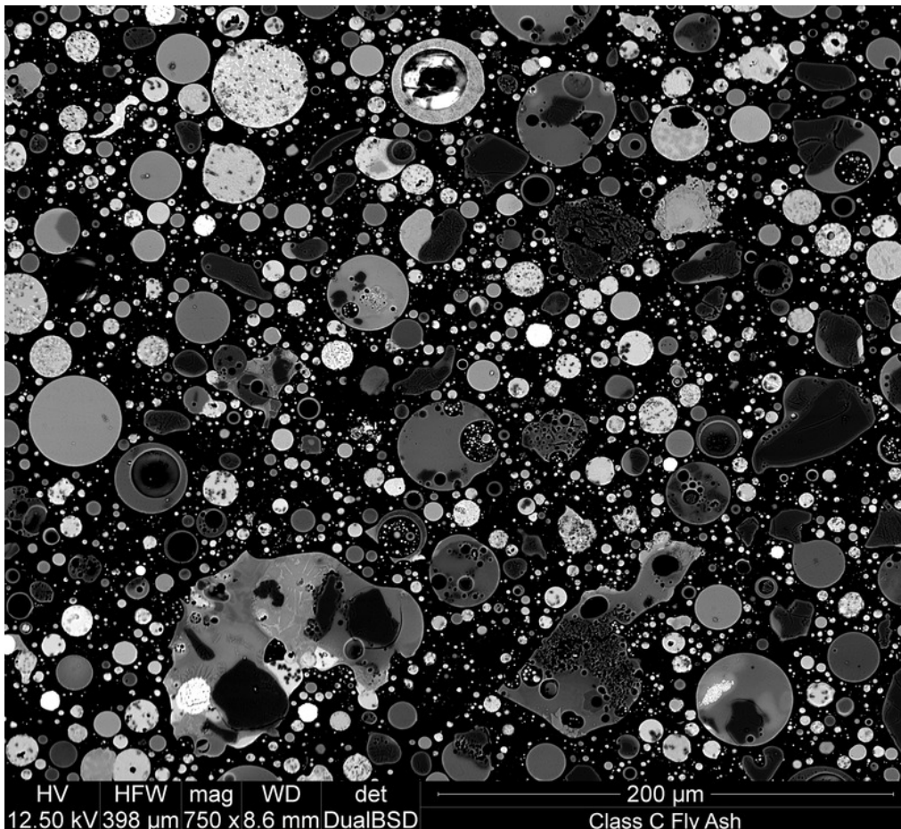
Photomicrograph made with a scanning electron microscope (SEM) and back-scatter detector: cross section of fly ash particles at 750x magnification (Licensed under CC BY-SA 3.0)
