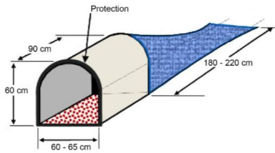
Tunnel souple
