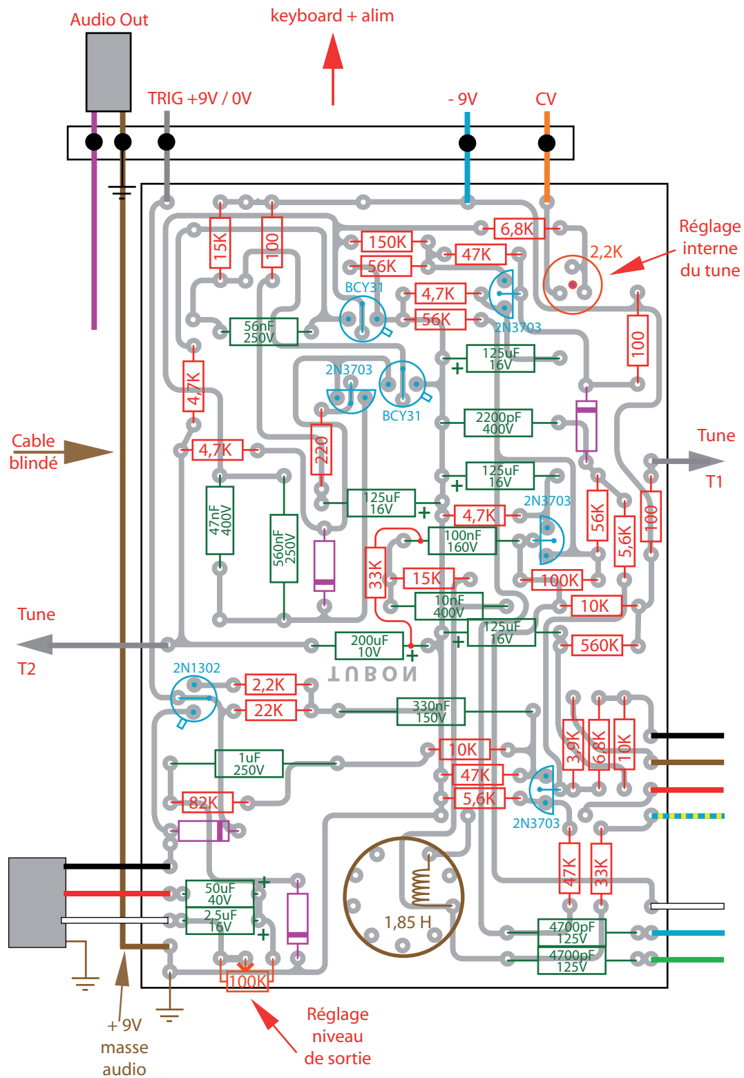
Platine composants
