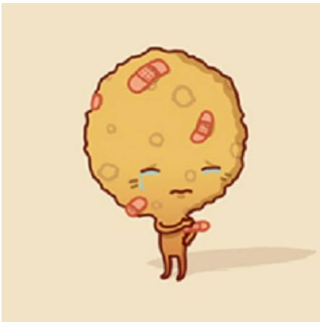
mercure
