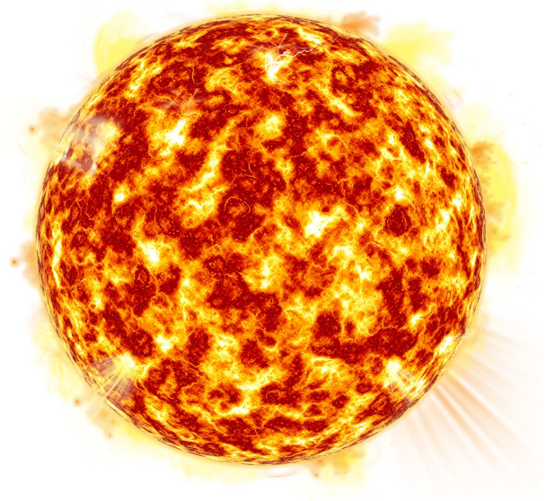
soleil
