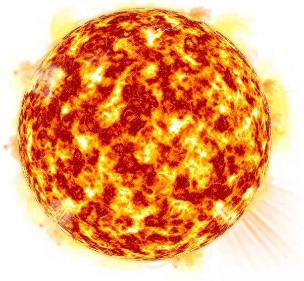
soleil
