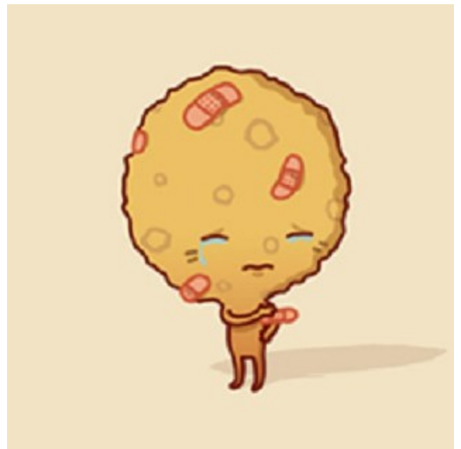
mercure
