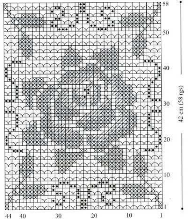
motif A (10 fs)
