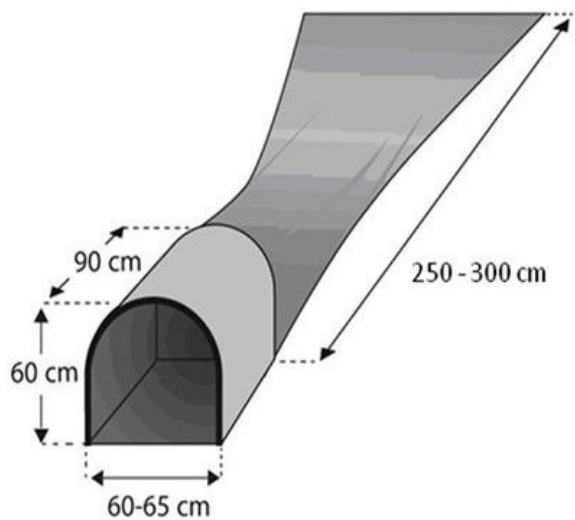
Tunnel souple
