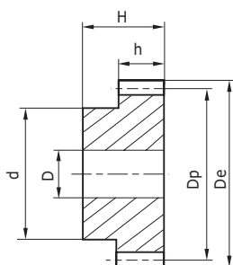
Module 1 ( h = 15 mm , H = 25 mm )
